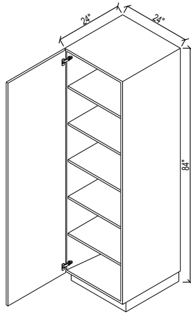
24TC8424
