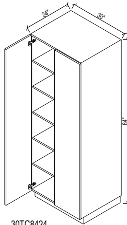
30TC8424
