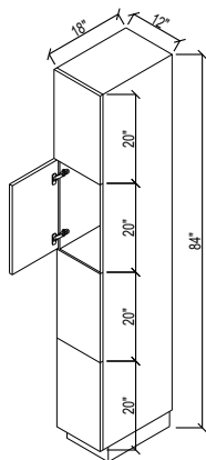
12 TC8418 3H
